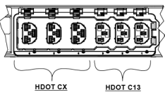
DETAIL A SCALE 0.36 : 1
