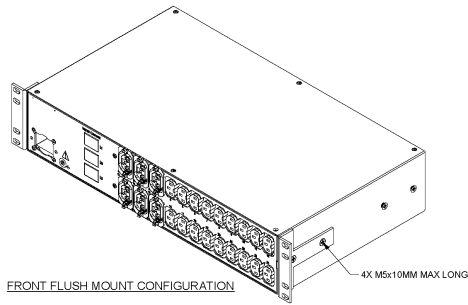
FRONT FLUSH MOUNT CONFIGURATION
