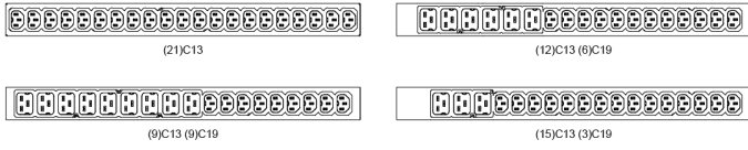
DETAIL A OPTIONAL OUTLET CONFIGURATIONS
